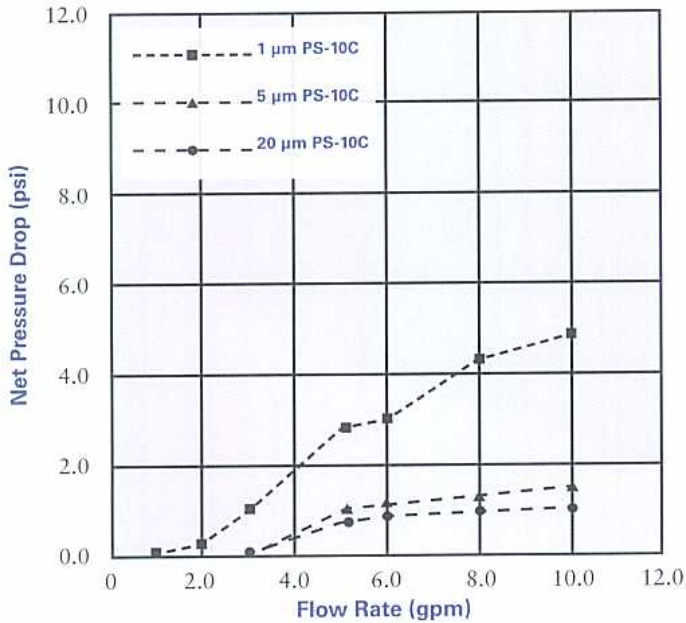
Net Pressure Drop vs. Flow Rate (water)
